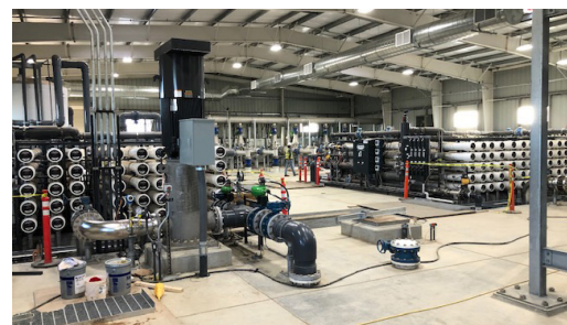
Expansion slot for reverse osmosis treatment skid
